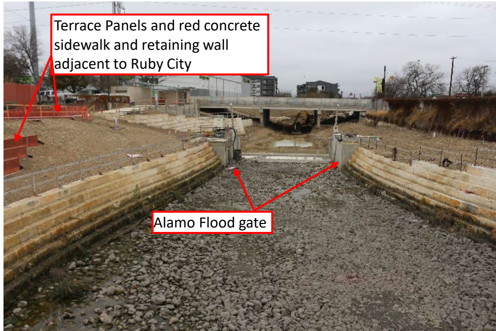
Phase 2 channel as seen from the Camp St. bridge facing south
